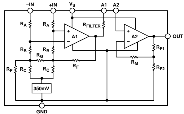
Figure 23. Simplified Schematic
