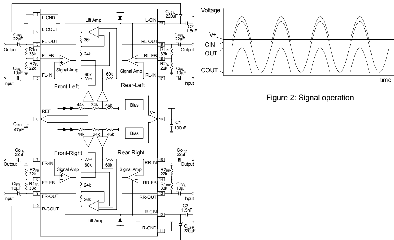
Figure 1: Block diagram and application circuit
