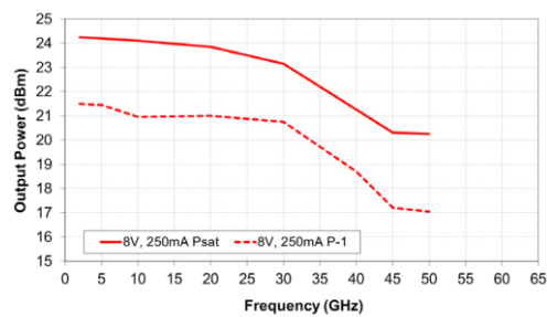
Output Power
