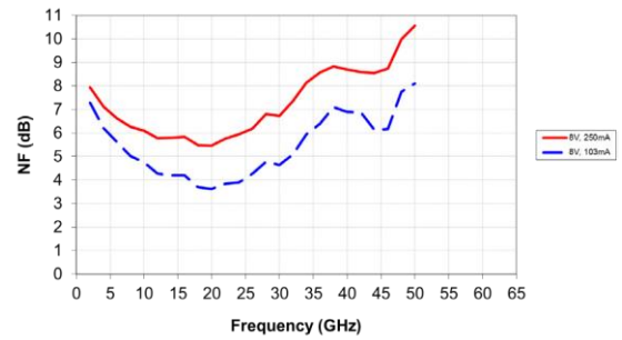
Noise Frequency
