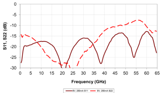
S11, S22
