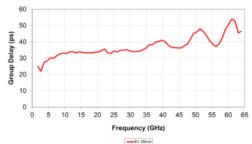
Group Delay
