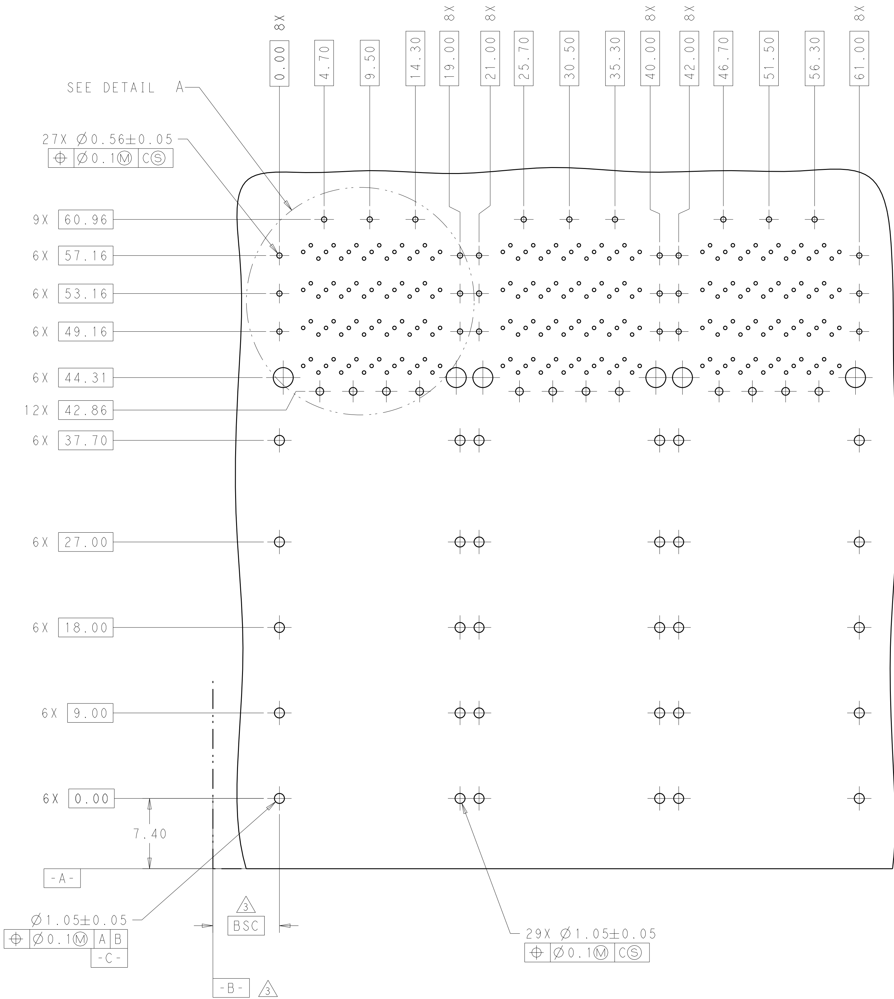
RECOMMENDED PC BOARD LAYOUT COMPONENT SIDE OF BOARD PCB TOLERANCE:±0.05
