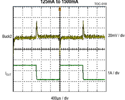
Load Transient Buck2 - Vout=1.5V 125mA to 1500mA
