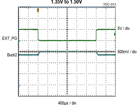
DVS Transition
