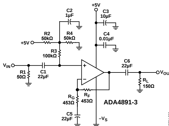
Figure 61. Single-Supply Video Driver Schematic
