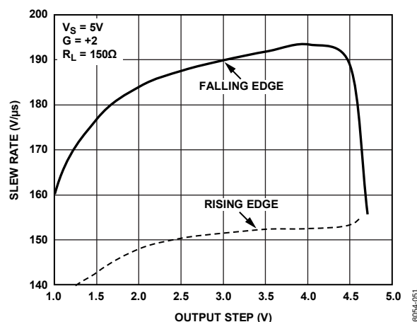
Figure 40. Slew Rate vs. Output Step
