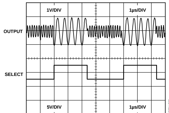
Figure 65. ADA4891-3 Mux Output
