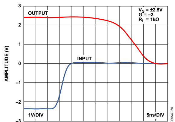
Figure 39. Output Overdrive Recovery from Positive Rail
