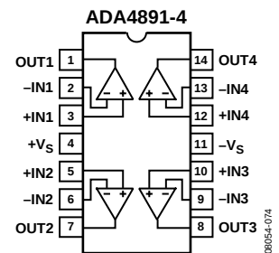
Figure 5. 14-Lead SOIC_N (R-14) and 14-Lead TSSOP (RU-14)
