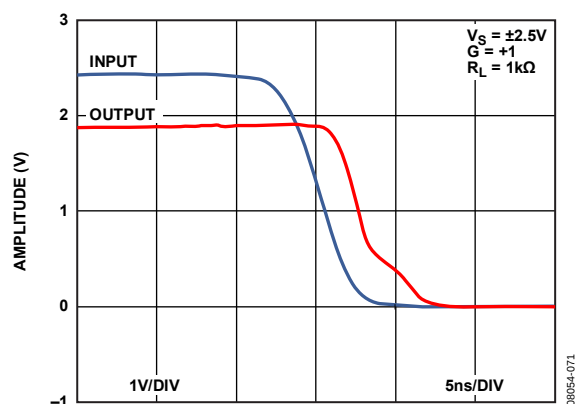
Figure 38. Input Overdrive Recovery from Positive Rail
