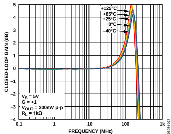
Figure 12. Small-Signal Frequency Response vs. Temperature, V_S = 5\text{ V} , ADA4891-3/ADA4891-4
