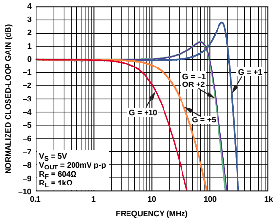
Figure 7. Small-Signal Frequency Response vs. Gain, V_S = 5\text{ V} , ADA4891-1/ADA4891-2
