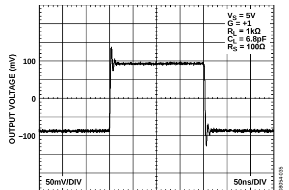
Figure 58. 200 mV Step Response, C_L = 6.8\text{ pF} , R_S = 100\Omega
