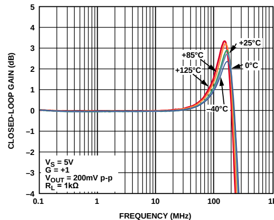
Figure 9. Small-Signal Frequency Response vs. Temperature, V_S = 5\text{ V} , ADA4891-1/ADA4891-2
