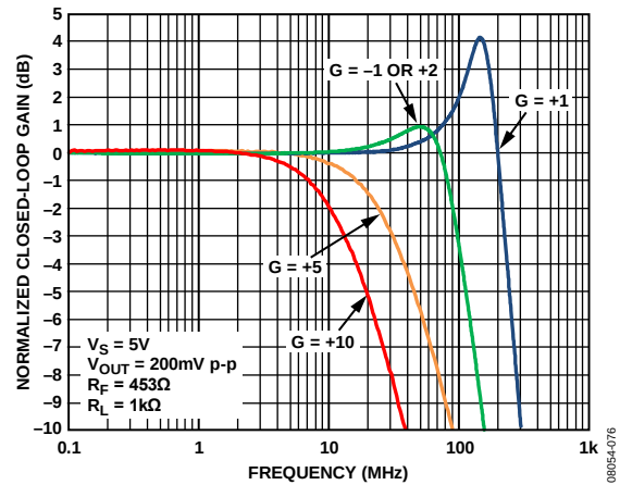
Figure 10. Small-Signal Frequency Response vs. Gain, V_S = 5\text{ V} , ADA4891-3/ADA4891-4
