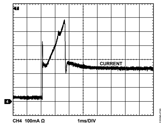
Figure 39. Transient Current Demand, Peak Demand
