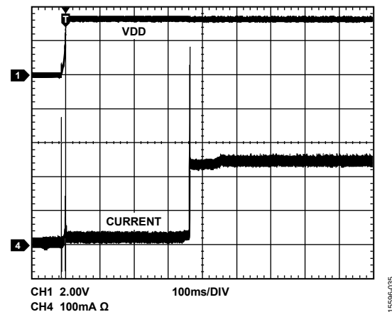
Figure 38. Transient Current Demand, Startup
