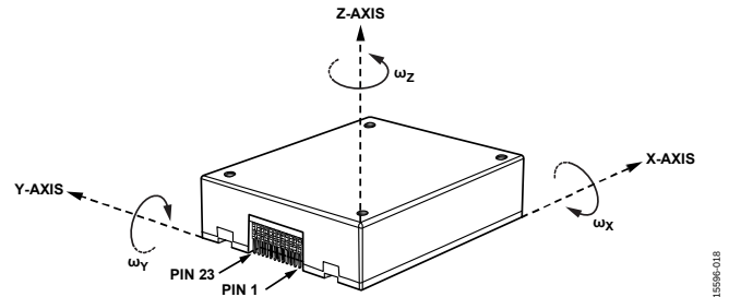
Figure 18. Gyroscopic Axis and Polarity Assignments
