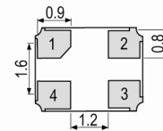
Underside View
