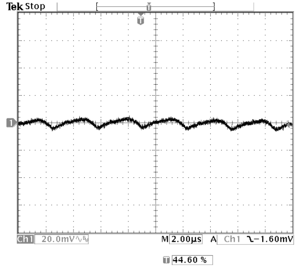
Fig-1.5V-5: Output voltage ripple (20mV/div.) for V_{out}=1.5V at full rated load current into a resistive load with external capacitance 47\mu F \times 2 ceramic + 1\mu F ceramic at V_{in}=12.0V . Time scale: 2us/div
