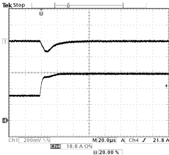
Fig-1.2V-6: Output voltage response for V_{out}=1.2V to positive load current step change from 15A to 30A with slew rate of 5A/\mu s at V_{in}=12V . C_o=47\mu F \times 2 ceramic. Top trace: output voltage (200mV/div.) Bottom trace: load current (10A/div.) Time scale: 20us/div.
