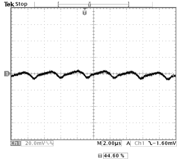
Fig-1.8V-5: Output voltage ripple (20mV/div.) for V_{out}=1.8V at full rated load current into a resistive load with external capacitance 47\mu F \times 2 ceramic + 1\mu F ceramic at V_{in}=12V . Time scale: 2 us/div
