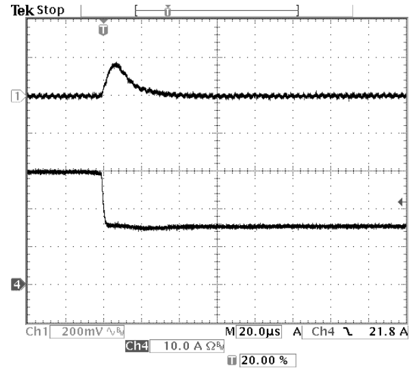
Fig-2.5V-7: Output voltage response for V_{out}=2.5V to negative load current step change from 30A to 15A with slew rate of -5A/us at V_{in}=12V . C_o=47uFx2 ceramic. Top trace: output voltage (200mV/div.) Bottom trace: load current (10A/div.) Time scale: 20us/div.
