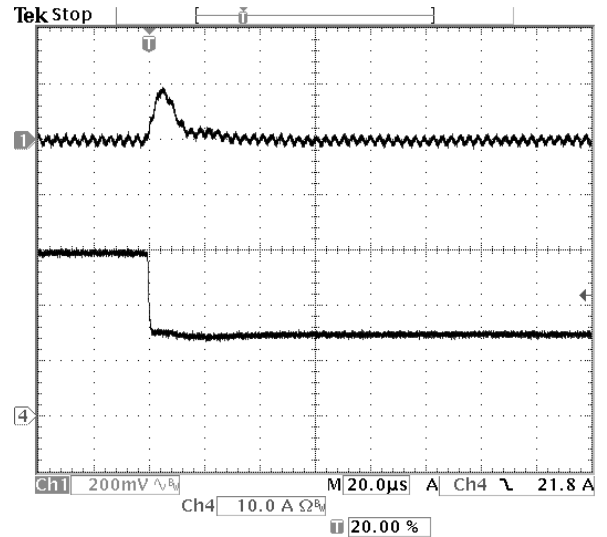
Fig-5.0V-7: Output voltage response for V_{out}=5.0V to negative load current step change from 30A to 15A with slew rate of -5A/\mu s at V_{in}=12V . C_o=47\mu F \times 2 ceramic. Top trace: output voltage (200mV/div.) Bottom trace: load current (10A/div.) Time scale: 20us/div.
