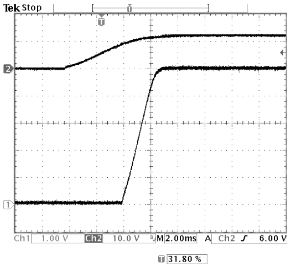
Fig-5.0V-4: Turn-on transient for V_{out}=5.0V with application of V_{in} at full rated load current (resistive) and 47\mu F \times 2 external capacitance at V_{in}=12V . Top trace: V_{in} (10V/div.) Bottom trace: output voltage (1V/div.) Time scale: 2 ms/div.
