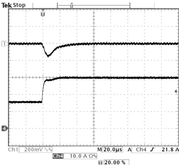
Fig-1.8V-6: Output voltage response for V_{out}=1.8V to positive load current step change from 15A to 30A with slew rate of 5A/\mu s at V_{in}=12V . C_o=47\mu F \times 2 ceramic. Top trace: output voltage (200mV/div.) Bottom trace: load current (10A/div.) Time scale: 20us/div.
