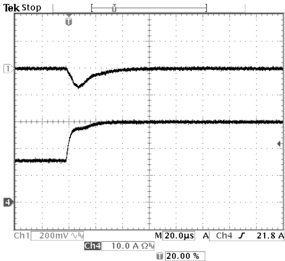
Fig-1.0V-6: Output voltage response for Vout=1.0V to positive load current step change from 15A to 30A with slew rate of 5A/us at Vin=12V. Co=47uFx2 ceramic. Top trace: output voltage (200mV/div.) Bottom trace: load current (10A/div.) Time scale: 20us/div.
