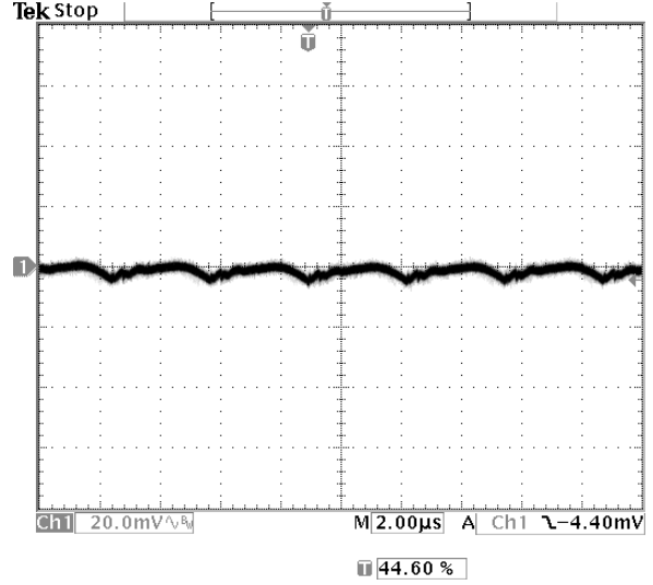
Fig-1.0V-5: Output voltage ripple (20mV/div.) for Vout=1.0V at full rated load current into a resistive load with external capacitance 47uFx2 ceramic + 1uF ceramic at Vin=12V. Time scale: 2 us/div
