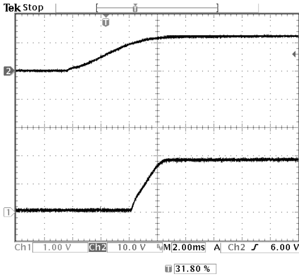
Fig-1.8V-4: Turn-on transient for V_{out}=1.8V with application of V_{in} at full rated load current (resistive) and 47\mu F \times 2 external capacitance at V_{in}=12V . Top trace: V_{in} (10V/div.) Bottom trace: output voltage (1V/div.) Time scale: 2 ms/div.
