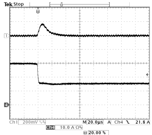
Fig-2.5V-7: Output voltage response for V_{out}=2.5V to negative load current step change from 30A to 15A with slew rate of -5A/\mu s at V_{in}=12V . C_o=47\mu F \times 2 ceramic. Top trace: output voltage (200mV/div.) Bottom trace: load current (10A/div.) Time scale: 20us/div.
