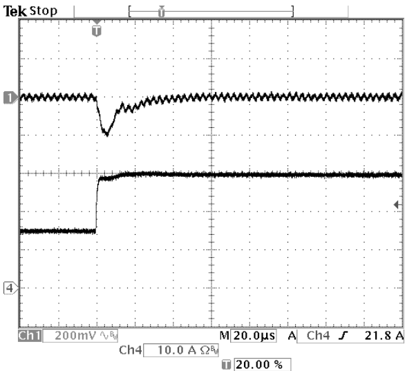
Fig-5.0V-6: Output voltage response for V_{out}=5.0V to positive load current step change from 15A to 30A with slew rate of 5A/\mu s at V_{in}=12V . C_o=47\mu F \times 2 ceramic. Top trace: output voltage (200mV/div.) Bottom trace: load current (10A/div.) Time scale: 20us/div.
