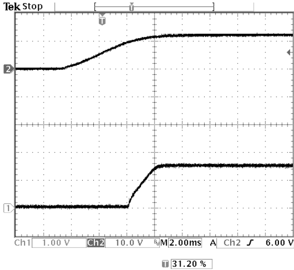
Fig-1.5V-4: Turn-on transient for V_{out}=1.5V with application of V_{in} at full rated load current (resistive) and 47\mu F \times 2 external capacitance at V_{in}=12V . Top trace: V_{in} (10V/div.) Bottom trace: output voltage (1V/div.) Time scale: 2 ms/div.
