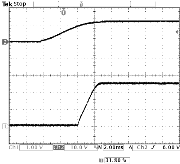
Fig-2.5V-4: Turn-on transient for V_{out}=2.5V with application of V_{in} at full rated load current (resistive) and 47uFx2 external capacitance at V_{in}=12V . Top trace: V_{in} (10V/div.) Bottom trace: output voltage (1V/div.) Time scale: 2 ms/div.
