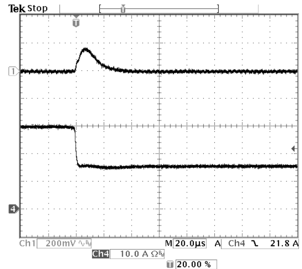
Fig-1.8V-7: Output voltage response for V_{out}=1.8V to negative load current step change from 30A to 15A with slew rate of -5A/\mu s at V_{in}=12V . C_o=47\mu F \times 2 ceramic. Top trace: output voltage (200mV/div.) Bottom trace: load current (10A/div.) Time scale: 20us/div.
