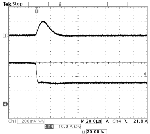
Fig-1.0V-7: Output voltage response for Vout=1.0V to negative load current step change from 30A to 15A with slew rate of -5A/us at Vin=12V. Co=47uFx2 ceramic. Top trace: output voltage (200mV/div.) Bottom trace: load current (10A/div.) Time scale: 20us/div.
