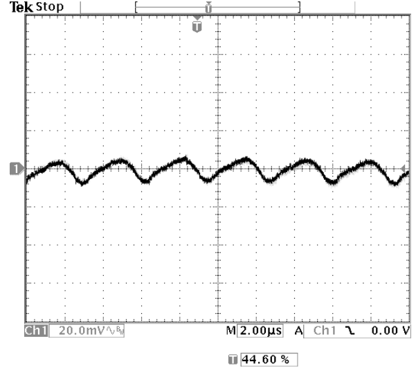
Fig-2.5V-5: Output voltage ripple (20mV/div.) for V_{out}=2.5V at full rated load current into a resistive load with external capacitance 47uFx2 ceramic + 1uF ceramic at V_{in}=12V . Time scale: 2 us/div
