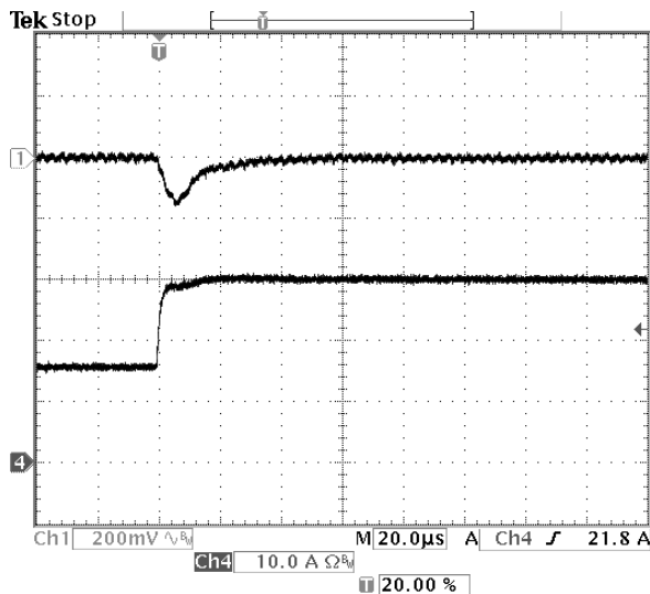
Fig-2.5V-6: Output voltage response for V_{out}=2.5V to positive load current step change from 15A to 30A with slew rate of 5A/\mu s at V_{in}=12V . C_o=47\mu F \times 2 ceramic. Top trace: output voltage (200mV/div.) Bottom trace: load current (10A/div.) Time scale: 20us/div.
