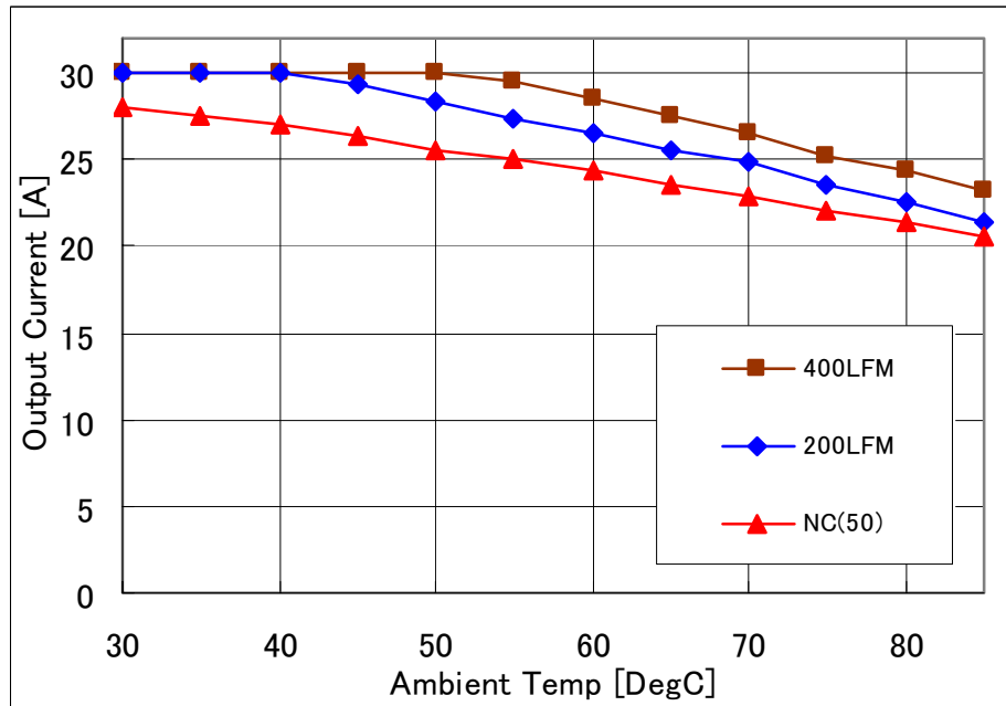
Fig-2.5V-1: Available load current vs. ambient temperature and airflow rates for Vout=2.5V with Vin=12V. Maximum component temperature ≤ 120°C
