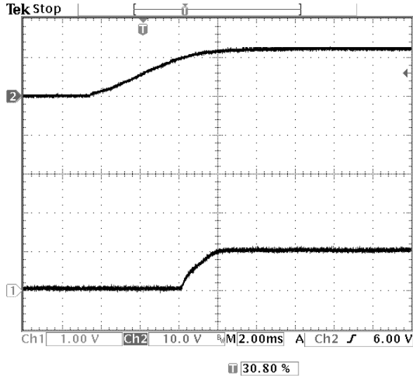
Fig-1.0V-4: Turn-on transient for Vout=1.0V with application of Vin at full rated load current (resistive) and 47uFx2 external capacitance at Vin=12V. Top trace: Vin (10V/div.) Bottom trace: output voltage (1V/div.) Time scale: 2 ms/div.
