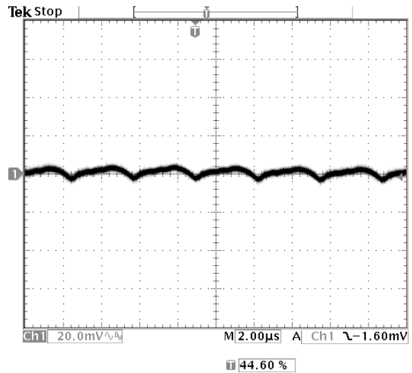
Fig-1.2V-5: Output voltage ripple (20mV/div.) for V_{out}=1.2V at full rated load current into a resistive load with external capacitance 47\mu F \times 2 ceramic + 1\mu F ceramic at V_{in}=12V . Time scale: 2us/div
