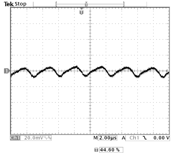
Fig-2.5V-5: Output voltage ripple (20mV/div.) for V_{out}=2.5V at full rated load current into a resistive load with external capacitance 47\mu F \times 2 ceramic + 1\mu F ceramic at V_{in}=12V . Time scale: 2 us/div
