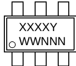
6-Lead SOT-23 (25AA02E64)
