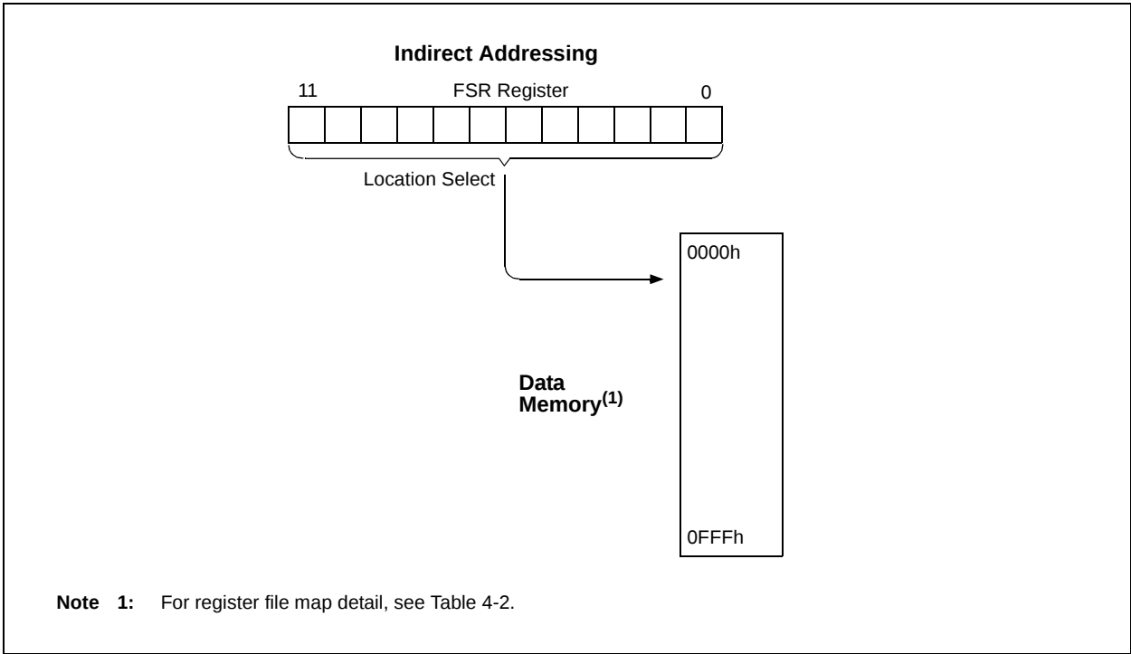
FIGURE 4-10: INDIRECT ADDRESSING
