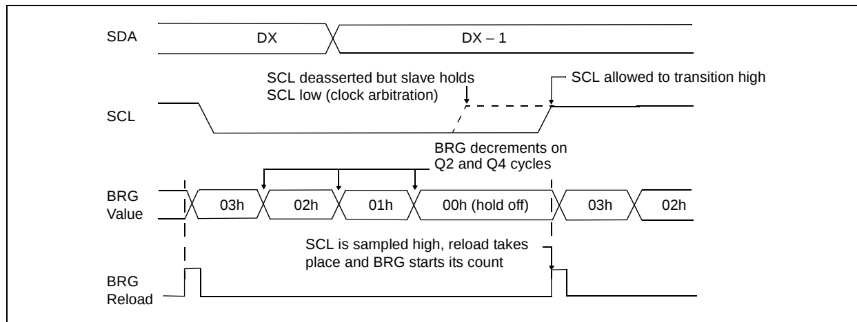
FIGURE 18-18: BAUD RATE GENERATOR TIMING WITH CLOCK ARBITRATION
