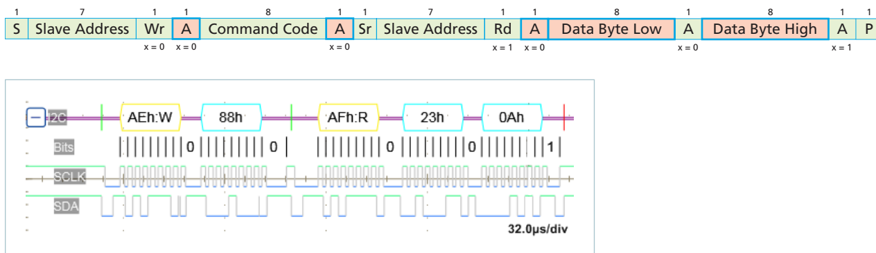
Figure 4 — MFR VIN MIN COMMAND (88h) READ WORD PROTOCOL
