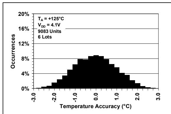
FIGURE 2-9: Temperature Accuracy Histogram at +125^{\circ}C .
