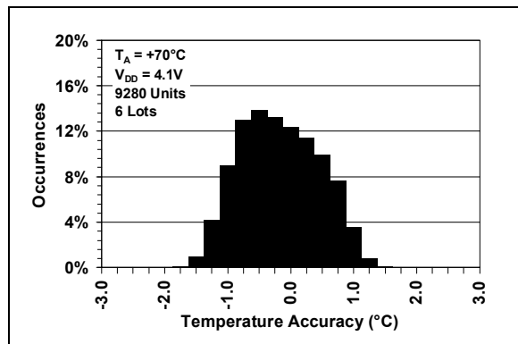
FIGURE 2-8: Temperature Accuracy Histogram at +70^{\circ}C .
