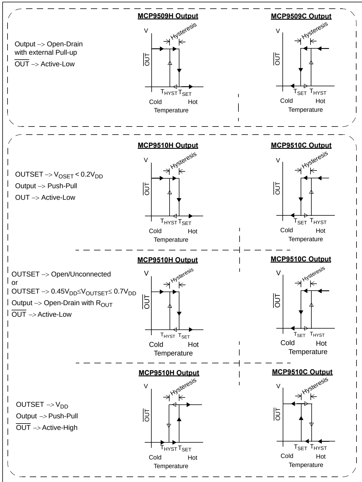
FIGURE 4-4: MCP9509/10 OUT/ \overline{\text{OUT}} Output Configuration.
