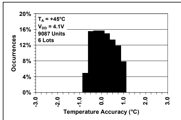
FIGURE 2-7: Temperature Accuracy Histogram at +45^{\circ}C .
