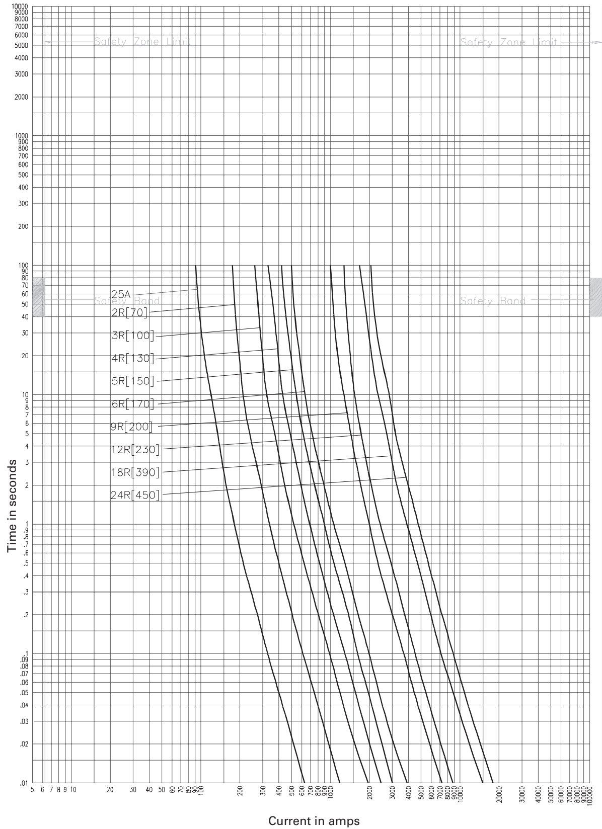
2.4kV time-current curves — minimum melting for 2HCLS- R and 2BCLS- R (25A, 2R-24R @25°C)
