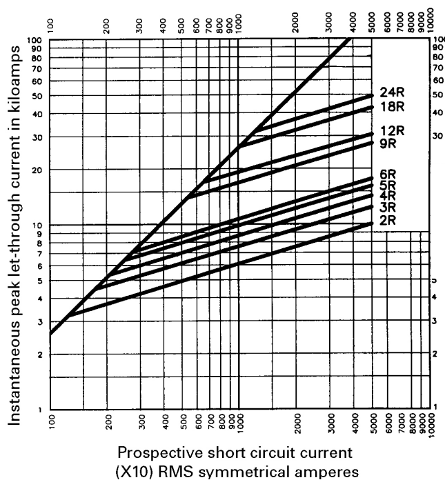
2.4kV peak let-through curves for JCK-_R and JCK-A-_R (2R- 24R @25°C)
