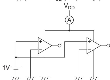
1. Supply Current, I_{DD} (Output High)
