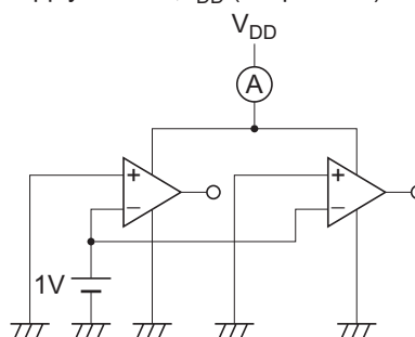
2. Supply Current, I_{DD} (Output Low)
