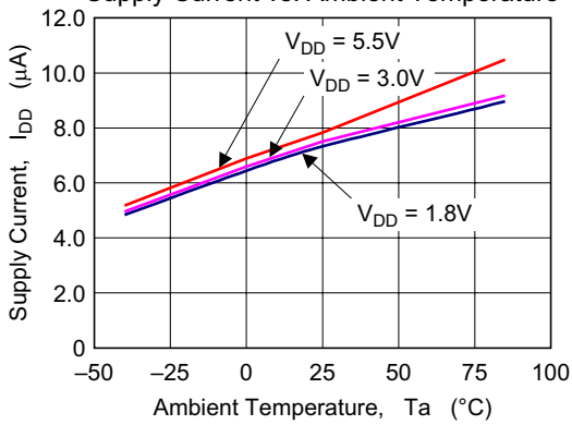
Figure 3-3 HA1631D03 Supply Current vs. Ambient Temperature
