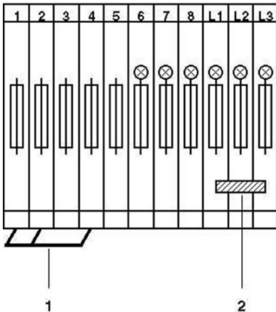
Circuit diagram
