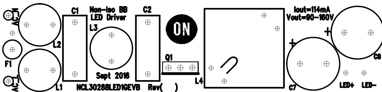
Figure 2. Top Silkscreen
