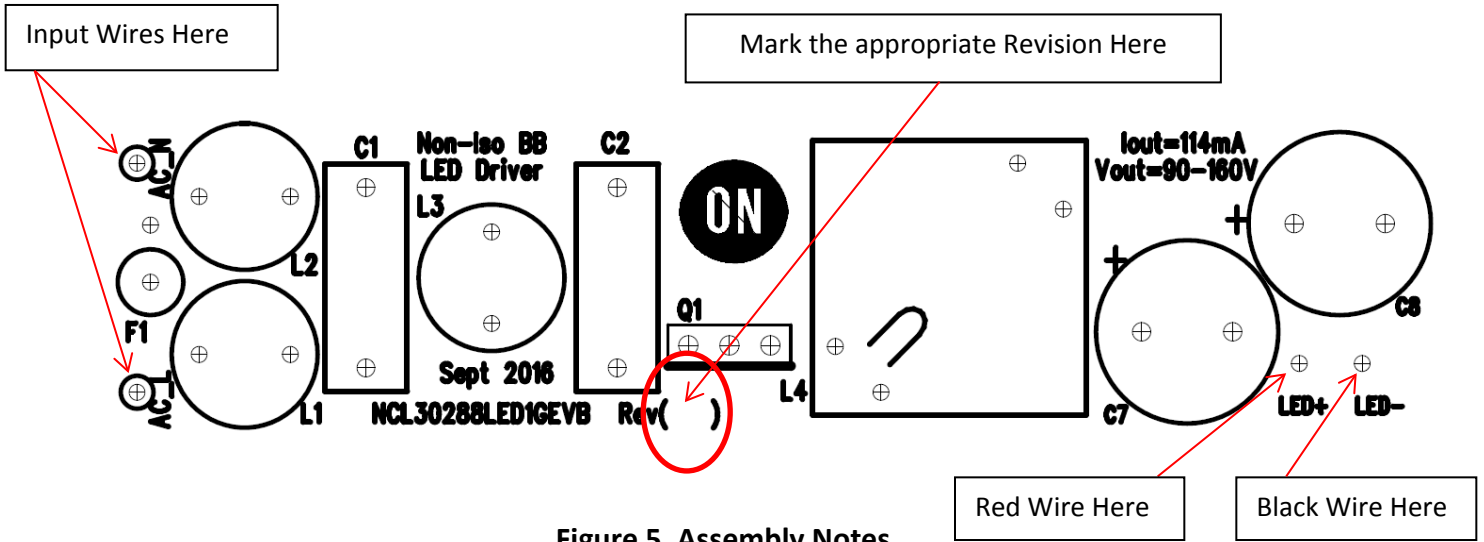
Figure 5. Assembly Notes
