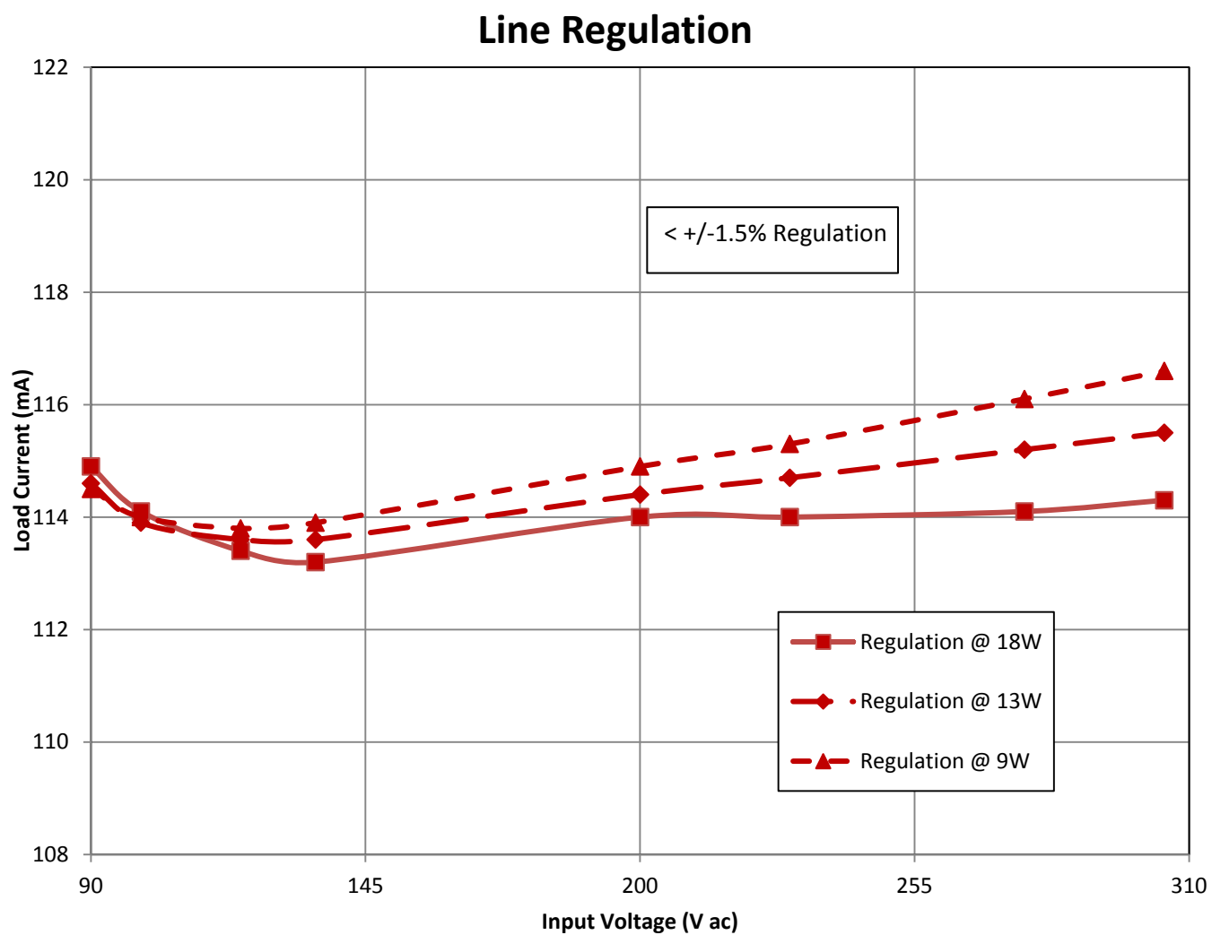
Figure 11. Line Regulation
