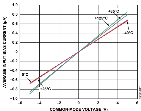
Figure 17. Average Input Bias Current vs. Common-Mode Voltage, -40^{\circ}C , +25^{\circ}C , +85^{\circ}C , +125^{\circ}C
