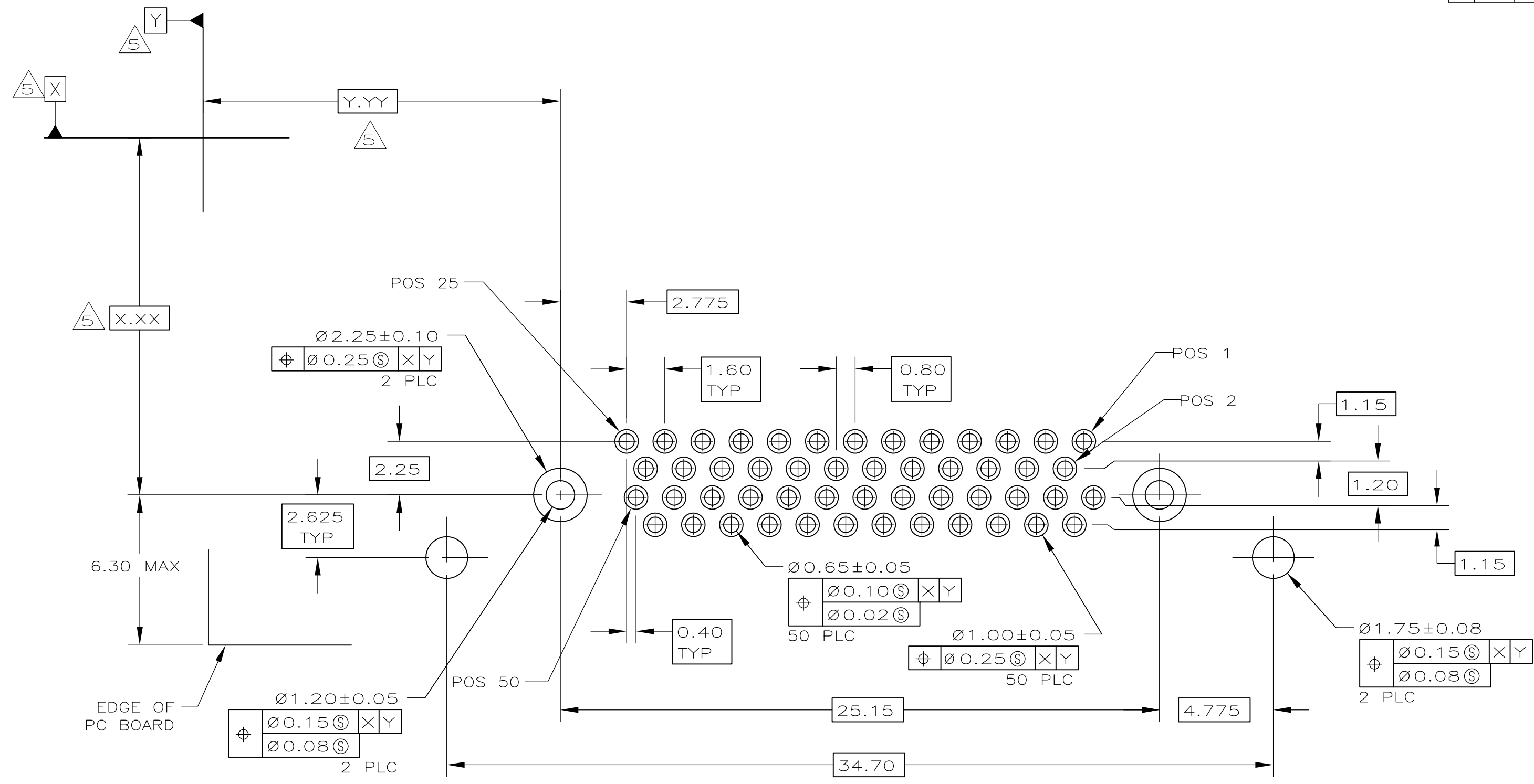
PC BOARD MOUNTING DIMENSIONS 3
