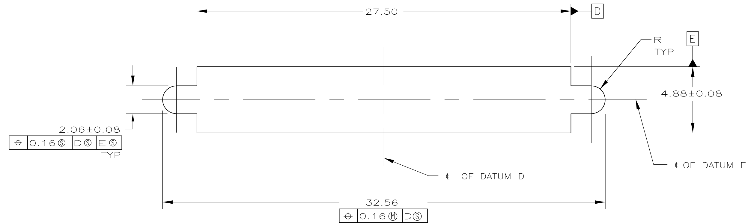
PANEL CUT-OUT DIMENSIONS 4
