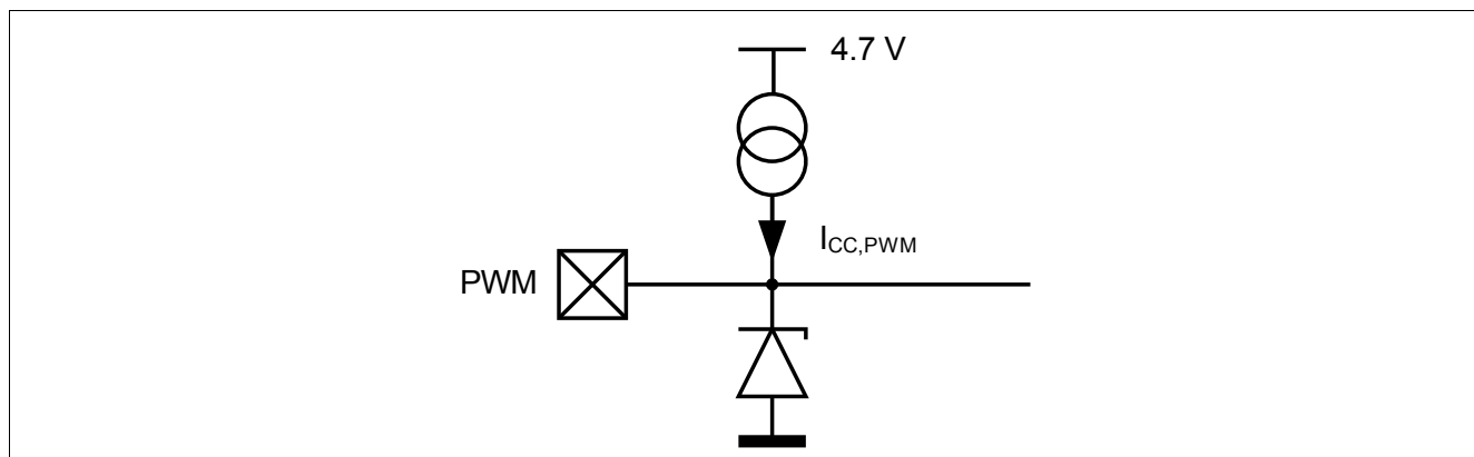
Figure 4 PWM Input
