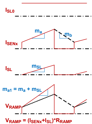
FIGURE 70. SLOPE COMPENSATION BLOCK DIAGRAM
