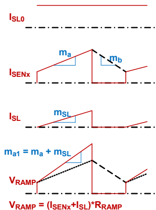
FIGURE 70. SLOPE COMPENSATION BLOCK DIAGRAM
