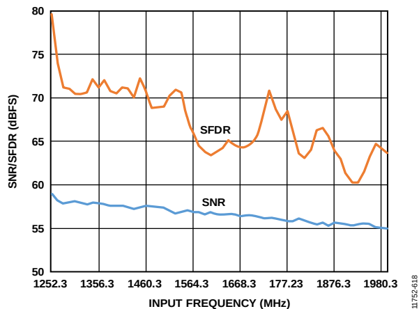
Figure 18. SNR/SFDR vs. f_{IN} ; 1.3 \text{ GHz} < f_{IN} < 2 \text{ GHz} ; Buffer Control 1 (0x018) = 8.5\times
