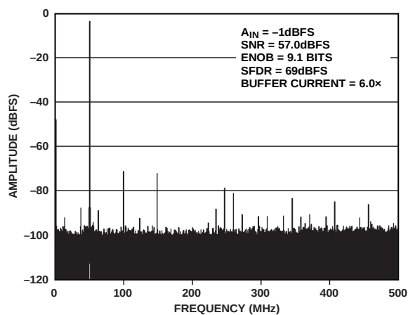
Figure 38. Single-Tone FFT with f_{IN} = 1950.3 MHz
