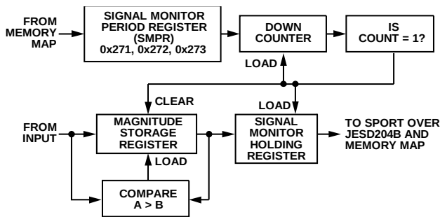
Figure 142. Signal Monitor Block
