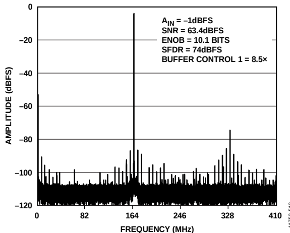
Figure 60. Single-Tone FFT with f_{IN} = 985.3 MHz
