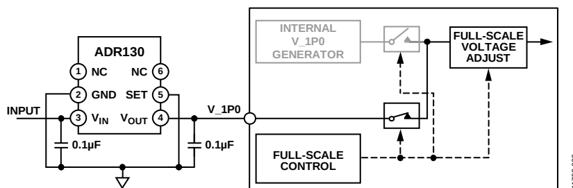
Figure 133. External Reference Using AD130
