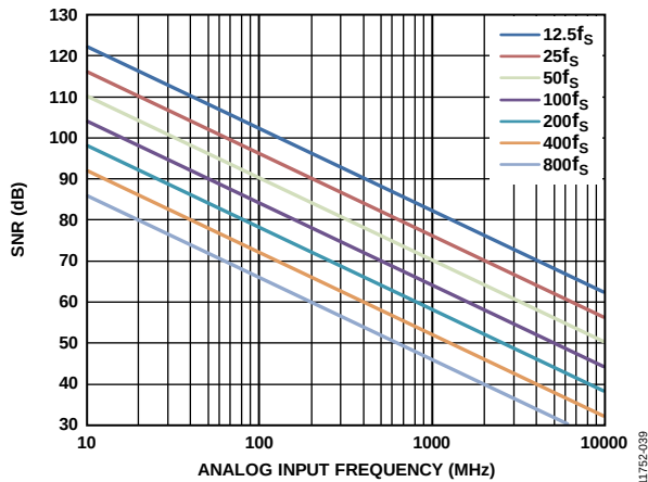
Figure 138. Ideal SNR vs. Input Frequency and Jitter
