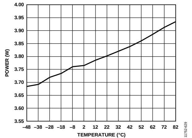
Figure 28. Power Dissipation vs. Temperature
