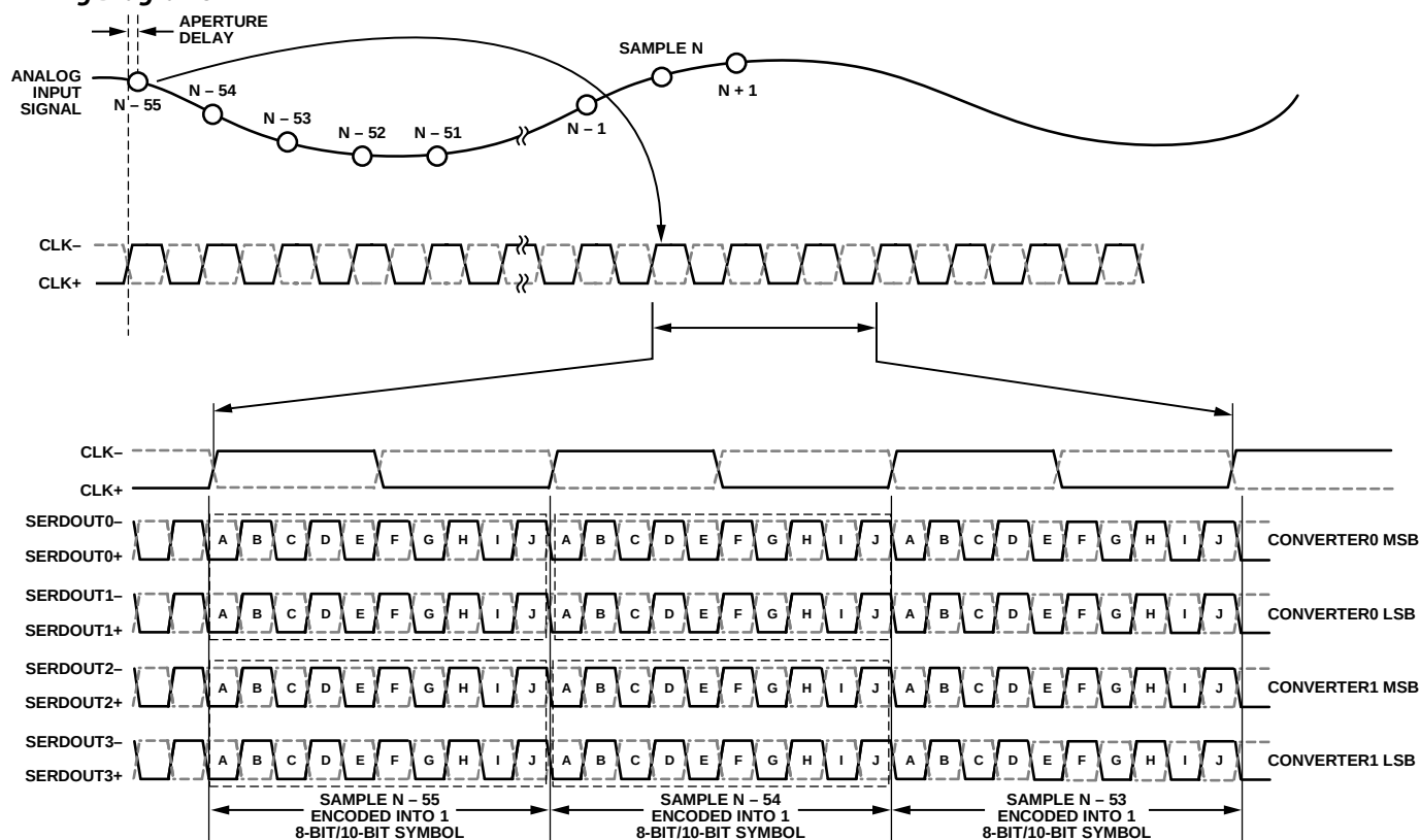
Figure 2. Data Output Timing (Full Bandwidth Mode; L = 4; M = 2; F = 1)
