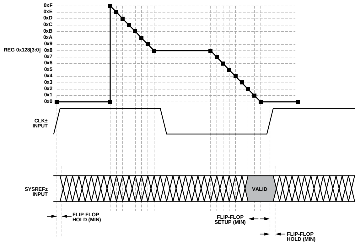
Figure 182. SYSREF± Setup Detector
