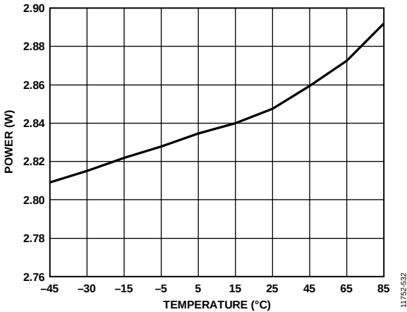
Figure 78. Power Dissipation vs. Temperature
