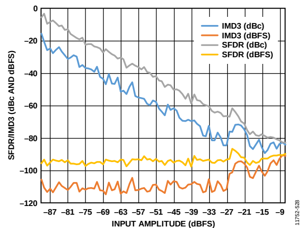
Figure 71. Two-Tone SFDR/IMD3 vs. Input Amplitude ( A_{IN} ) with f_{IN1} = 184 MHz and f_{IN2} = 187 MHz
