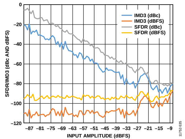
Figure 72. Two-Tone IMD3/SFDR vs. Input Amplitude ( A_{IN} ) with f_{IN1} = 338 MHz and f_{IN2} = 341 MHz
