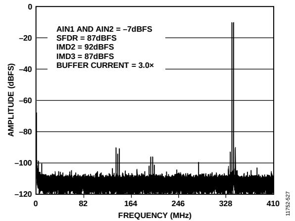
Figure 70. Two-Tone FFT; f_{IN1} = 338 MHz, f_{IN2} = 341 MHz
