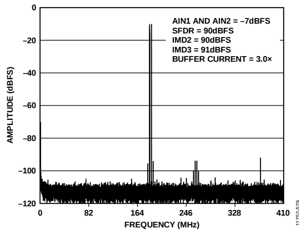
Figure 69. Two-Tone FFT; f_{IN1} = 184 MHz, f_{IN2} = 187 MHz
