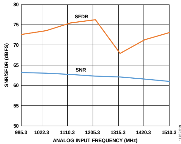
Figure 67. SNR/SFDR vs. f_{IN} ; 1 GHz < f_{IN} < 1.5 GHz; Buffer Control 1 (0x018) = 6.5x
