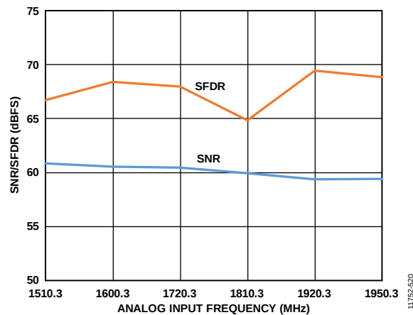
Figure 68. SNR/SFDR vs. f_{IN} ; 1.5 GHz < f_{IN} < 2 GHz; Buffer Control 1 (0x018) = 8.5x
