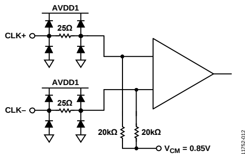
Figure 105. Clock Inputs
