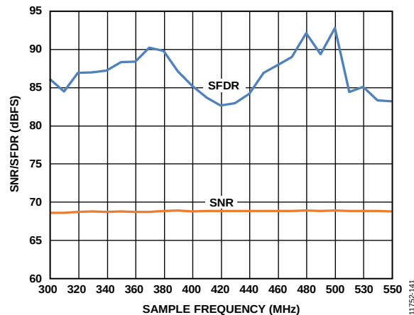
Figure 89. SNR/SFDR vs. f_s , f_{IN} = 170.3 MHz; Buffer Control 1 = 2.0\times
