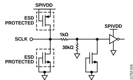
Figure 109. SCLK Input
