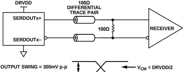
Figure 160. DC-Coupled Digital Output Termination Example
