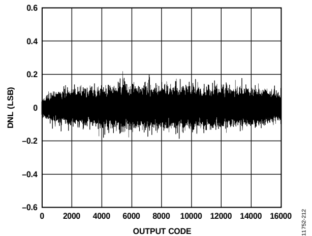
Figure 51. DNL, f_{IN} = 15 MHz
