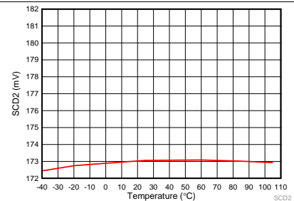
Figure 10. Short Circuit Charge Protection Threshold vs. Temperature
