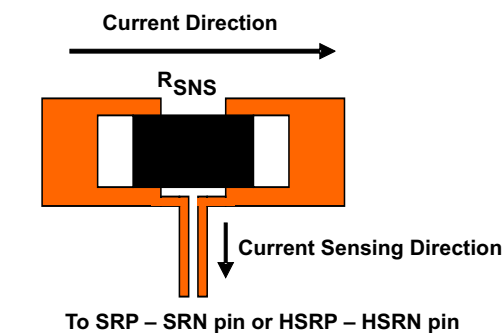
Figure 26. Sensing Resistor PCB Layout
