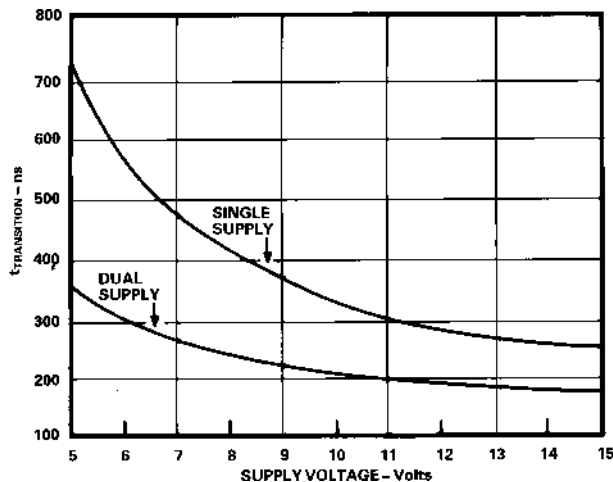
Figure 3. t_{\text{TRANSITION}} vs. Supply Voltage: Dual and Single Supplies, T_A = +25^\circ\text{C} (Note: For V_{DD} and |V_{SS}| < 10\text{ V} ; V1 = V_{DD}/V_{SS} , V2 = V_{SS}/V_{DD} . See Test Circuit 6)
