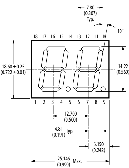
14.2 mm (0.56”) Dual Digit Displays Package Dimension
