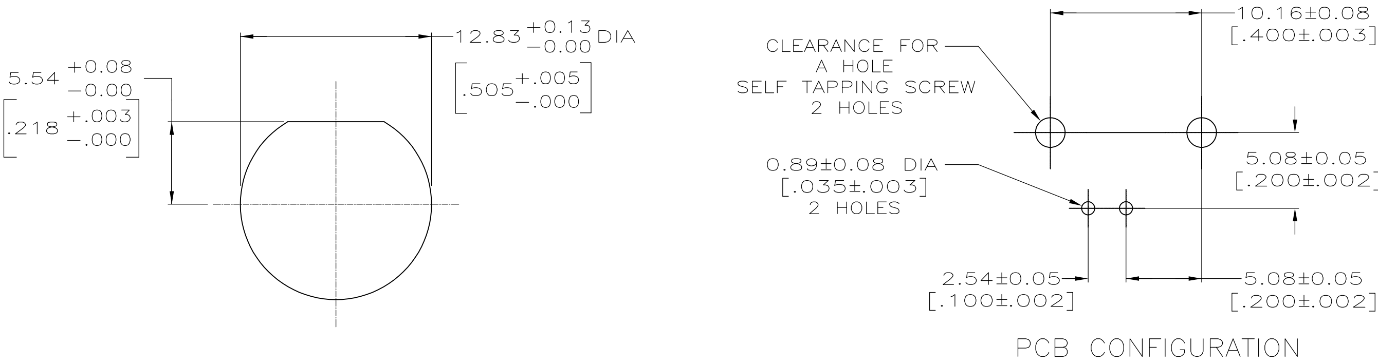
RECOMMENDED PANEL CUTOUT
