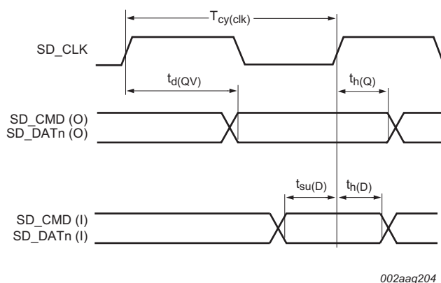
Fig 37. SD/MMC timing
