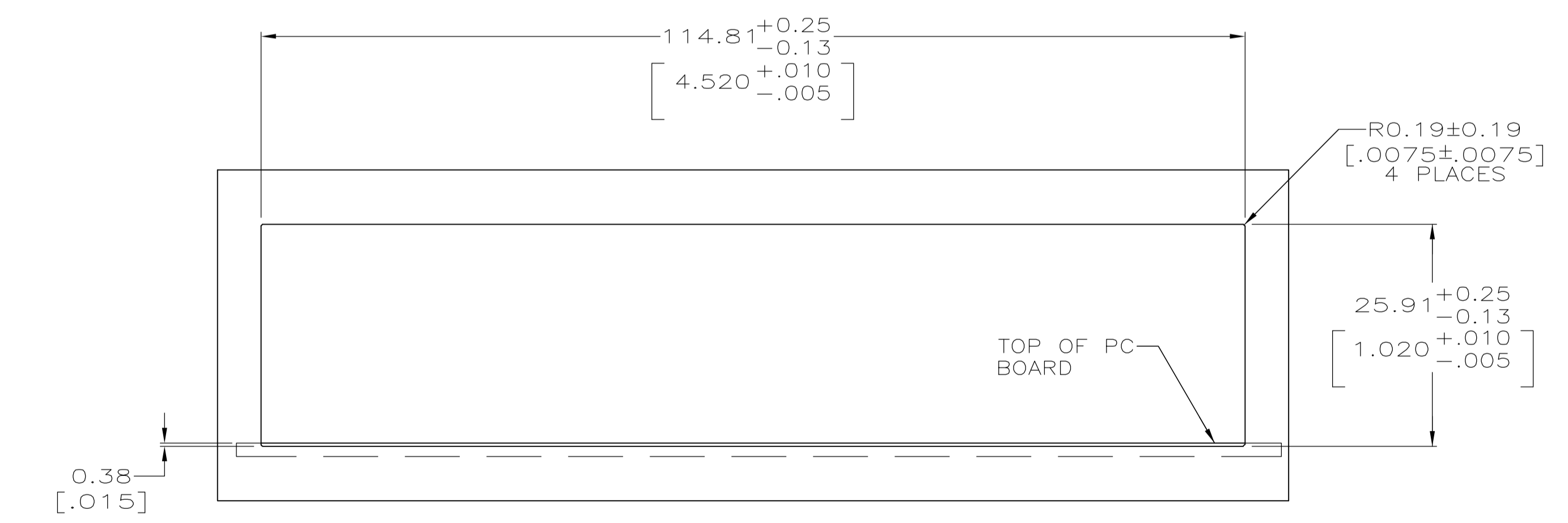
SUGGESTED PANEL CUTOUT DIMENSIONS SCALE 2:1
