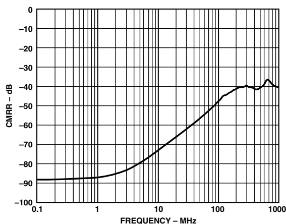
TPC 24. CMRR vs. Frequency; V_S = \pm 6 V or V_S = \pm 2.5 V
