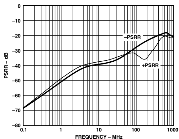
TPC 27. PSRR vs. Frequency; V_S = \pm 6 V or V_S = \pm 2.5 V
