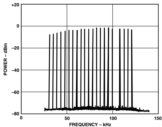
TPC 23. Multitone Power Ratio: V_S = \pm 6 V, 13 dBm Output Power into 25\ \Omega
