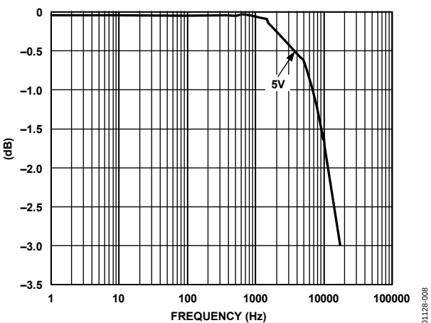
Figure 8. Typical Bandwidth
