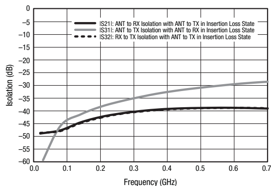
Figure 6. Isolation vs Frequency (ANT to RX, TX to RX, and ANT to TX Ports; V_{CTL} = 5\text{ V} , I_{CTL} = -50\text{ mA} )
