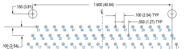
51 PIN MWDM-51PBR
