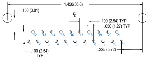
21 SOCKET MWDM-21SBR
