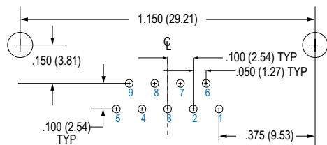
9 PIN MWDM-9PBR
