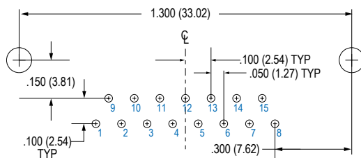
15 SOCKET MWDM-15SBR
