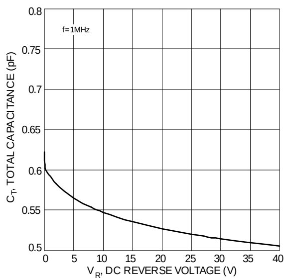
Fig. 4 Total Capacitance vs. Reverse Voltage, Per Element
