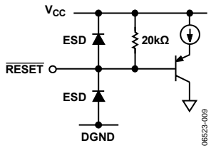
Figure 9. Reset Input
