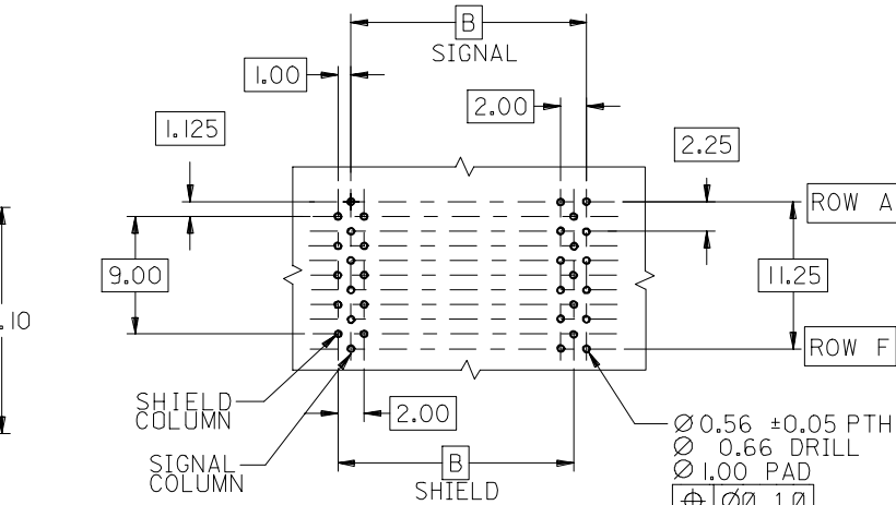
BACKPLANE HOLE PATTERN RECOMMENDED DIMENSIONS
