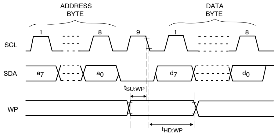
Figure 9. WP Timing
