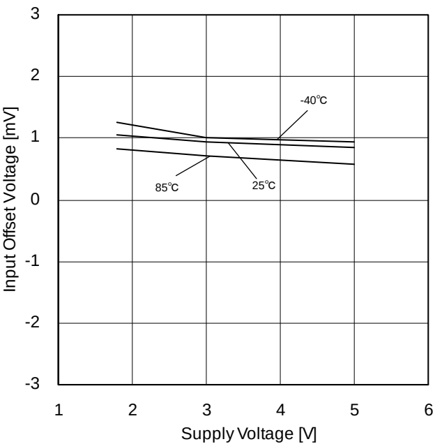
Figure 38. Input Offset Voltage vs Supply Voltage
