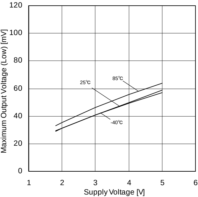
Figure 10. Maximum Output Voltage (Low) vs Supply Voltage ( R_L=2k\Omega )
