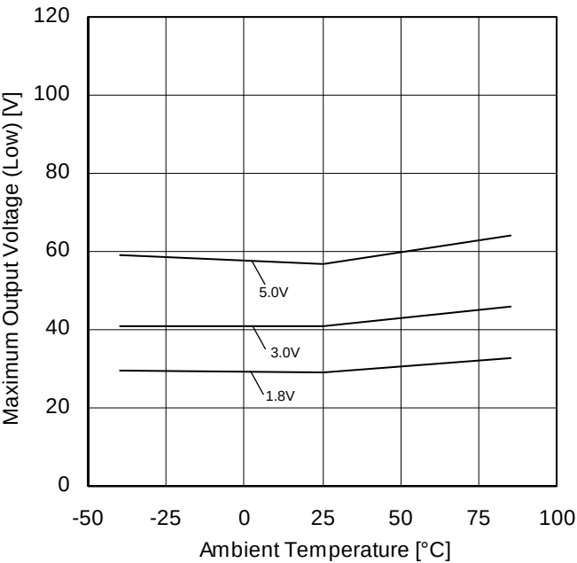
Figure 11. Maximum Output Voltage (Low) vs Ambient Temperature ( R_L=2k\Omega )
