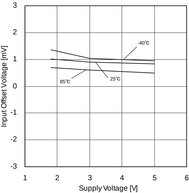
Figure 12. Input Offset Voltage vs Supply Voltage
