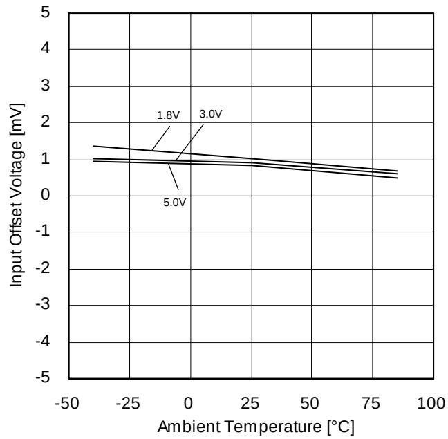
Figure 13. Input Offset Voltage vs Ambient Temperature
