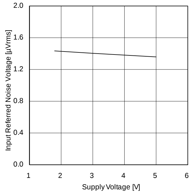
Figure 51. Input Referred Noise Voltage vs Supply Voltage ( T_A=25^\circ\text{C} )
