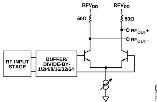
Figure 21. Output Stage
