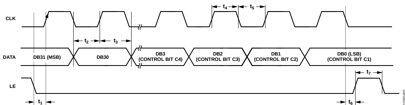
Figure 2. Timing Diagram
