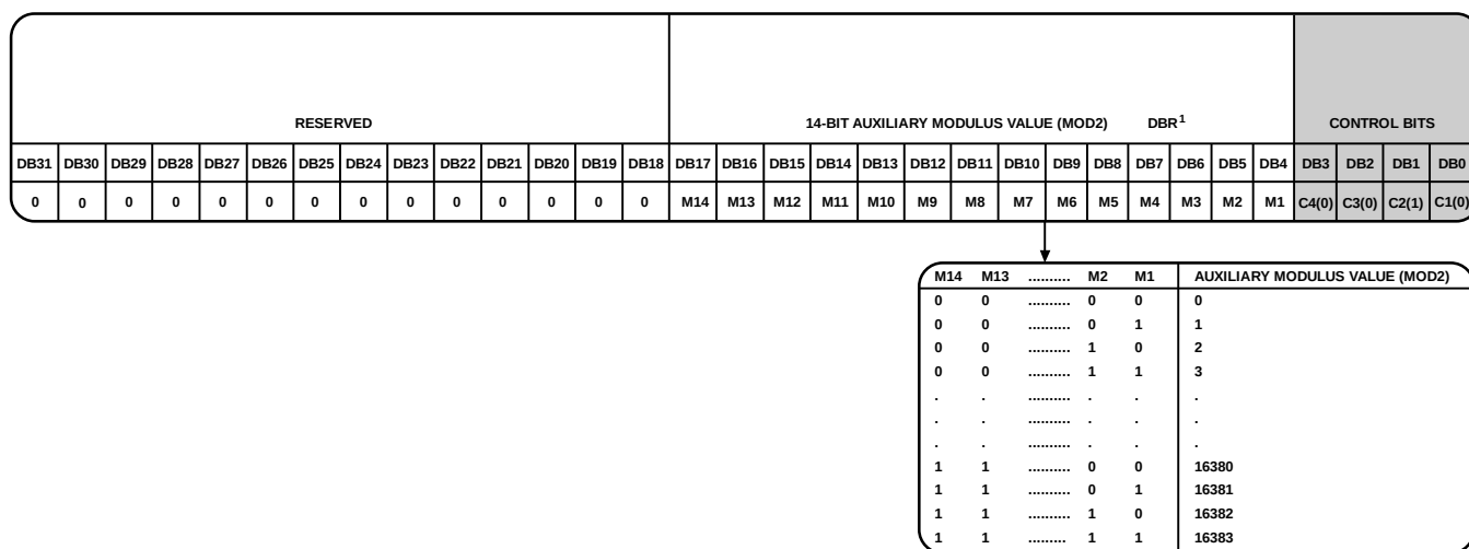
Figure 26. Register 2 (R2)
