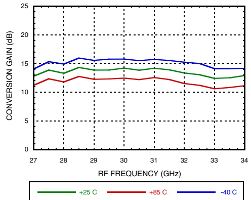
Conversion Gain vs. Temperature, LSB
