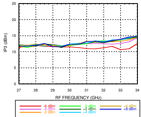
Output IP3 vs. LO Drive, USB
