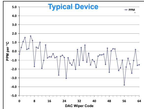
FIGURE 2-64: V_{OUT} Tempco vs. Code ( ((V_{OUT(+125C)} - V_{OUT(-40C)}) / V_{OUT(+25C, Code=FS)}) / 165) * 1,000,000 ), V_{DD} = 3.0\text{V} , V_{REF} = 1.0\text{V} .
