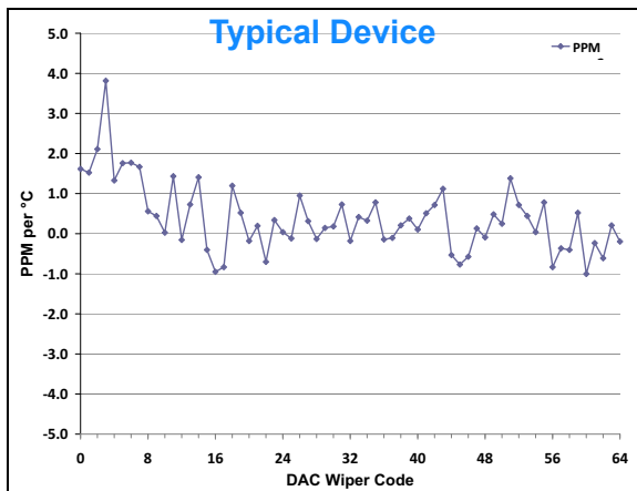
FIGURE 2-63: V_{OUT} Tempco vs. Code ( ((V_{OUT(+125C)} - V_{OUT(-40C)}) / V_{OUT(+25C, Code=FS)}) / 165) * 1,000,000 ), V_{DD} = 3.0\text{V} , V_{REF} = 1.65\text{V} .
