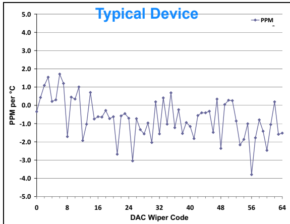
FIGURE 2-61: V_{OUT} Tempco vs. Code ( ((V_{OUT(+125C)} - V_{OUT(-40C)}) / V_{OUT(+25C, Code=FS)}) / 165) * 1,000,000 ), V_{DD} = 3.6\text{V} , V_{REF} = 1.0\text{V} .
