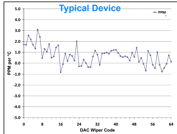
FIGURE 2-65: V_{OUT} Tempco vs. Code ( ((V_{OUT(+125C)} - V_{OUT(-40C)}) / V_{OUT(+25C, Code=FS)}) / 165) * 1,000,000 ), V_{DD} = 2.7\text{V} , V_{REF} = 1.65\text{V} .
