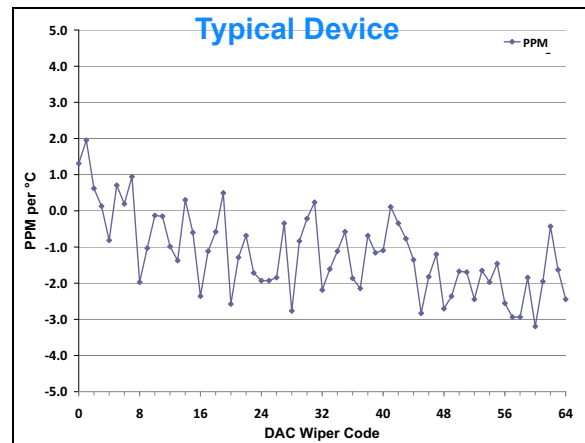
FIGURE 2-66: V_{OUT} Tempco vs. Code ( ((V_{OUT(+125C)} - V_{OUT(-40C)}) / V_{OUT(+25C, Code=FS)}) / 165) * 1,000,000 ), V_{DD} = 2.7\text{V} , V_{REF} = 1.0\text{V} .
