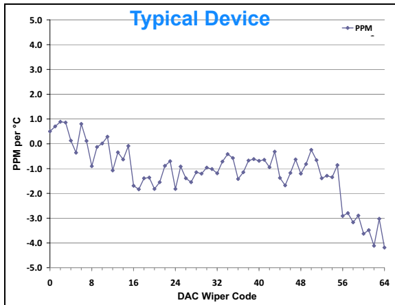
FIGURE 2-62: V_{OUT} Tempco vs. Code ( ((V_{OUT(+125C)} - V_{OUT(-40C)}) / V_{OUT(+25C, Code=FS)}) / 165) * 1,000,000 ), V_{DD} = 3.0\text{V} , V_{REF} = 3.0\text{V} .
